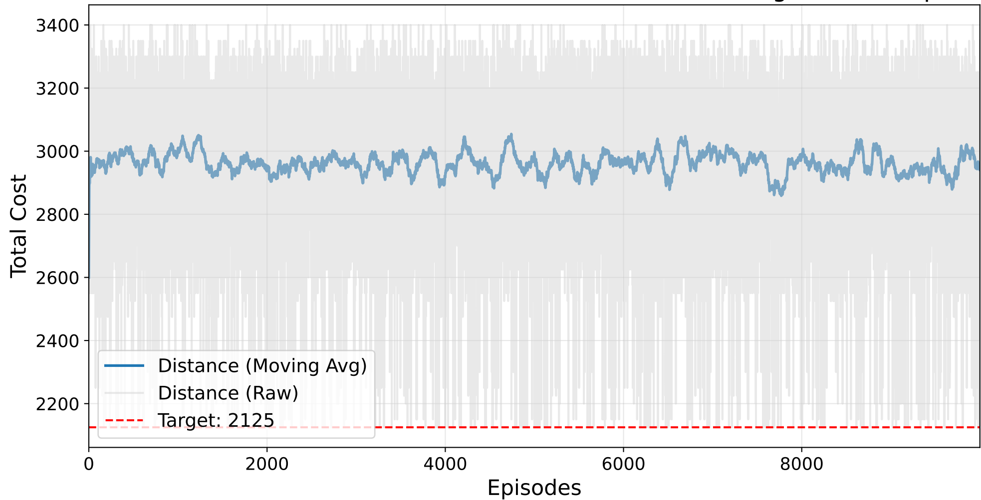
Final GAUSSIAN PROCESS Masked AutoRL-SOP Training - ESC07.sop
